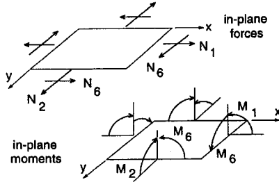
Fig. 2 Geometry of in-plane force and moment resultants.
