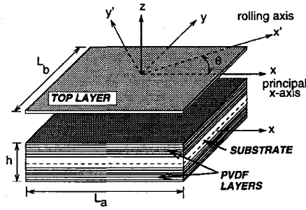
Fig. 1 Geometry of general piezoelectric laminate system.
