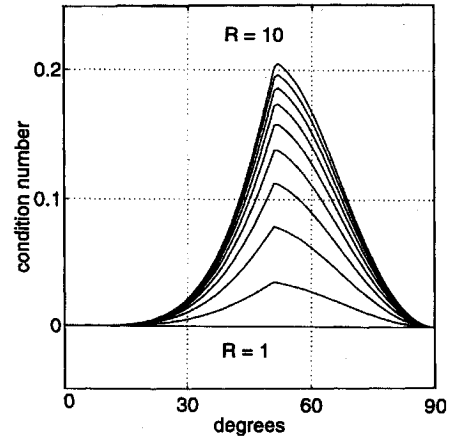
Fig. A1 Reciprocal condition number N_r as a function of the angle \gamma ; plots are given for all integer values of R between 1 and 10.
